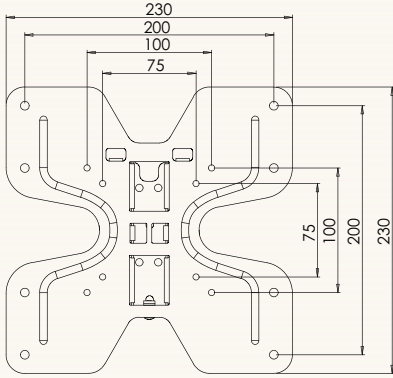
VESA Details
